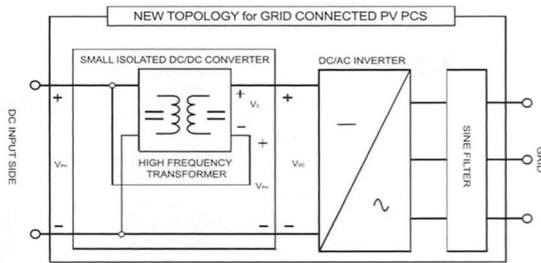
Fig. 3 Proposed topology for PV PCS
