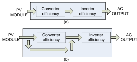
Fig. 5 Efficiency flow diagram (a) conventional DC/DC converter + inverter topology, (b) proposed topology
