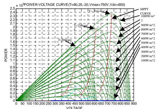
Fig. 2 Characteristics of PV module
