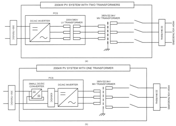
Fig. 6 Comparison to the two topologies (a) using low voltage line frequency transformer (b) using proposed topology
