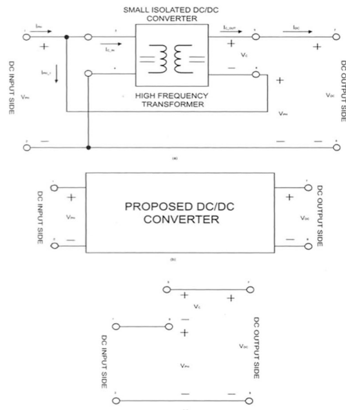
Fig. 4 Explanatory diagram of the proposed topology (a) main block diagram, (b) input/output block diagram, (c) the concept of the proposed topology
