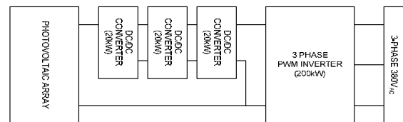
Fig. 7 System diagram of 250kW grid connected PV PCS
