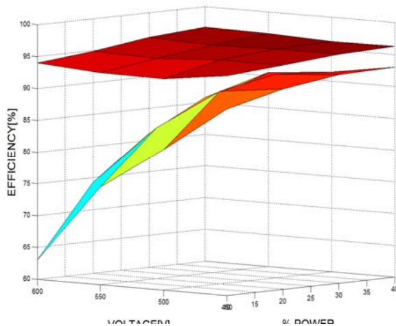
Fig. 11 Experimental total system efficiency curve
