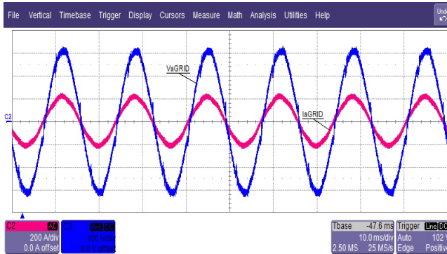
Fig. 10 Experimental waveforms (blue : grid voltage, 100V/div, red : inverter output current, 200A/div)
