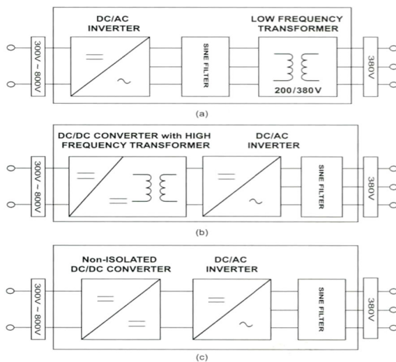
Fig. 1 The topologies of photovoltaic PCS
